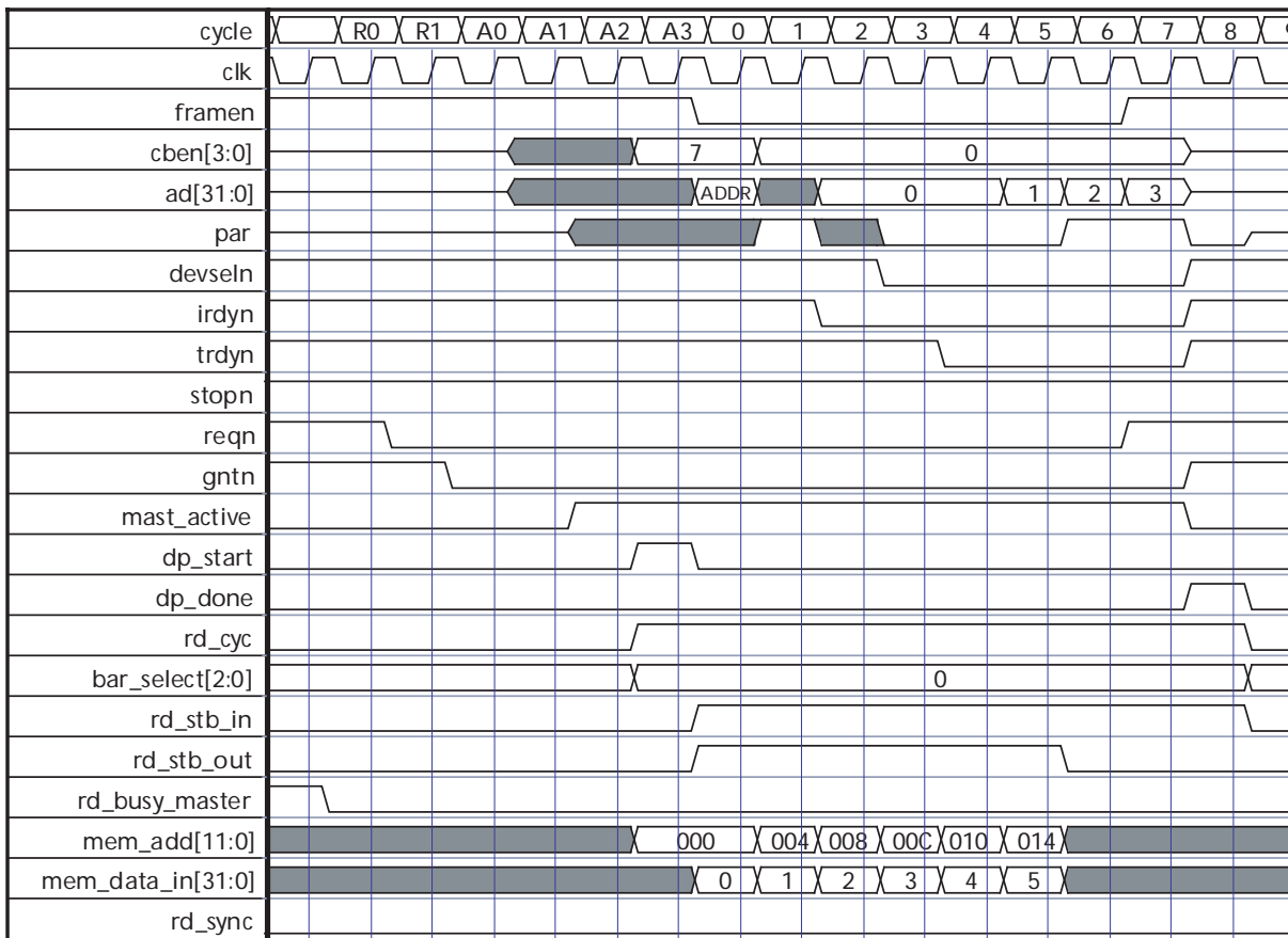
Figure 6-43 · RD_BUSY_MASTER Operation
