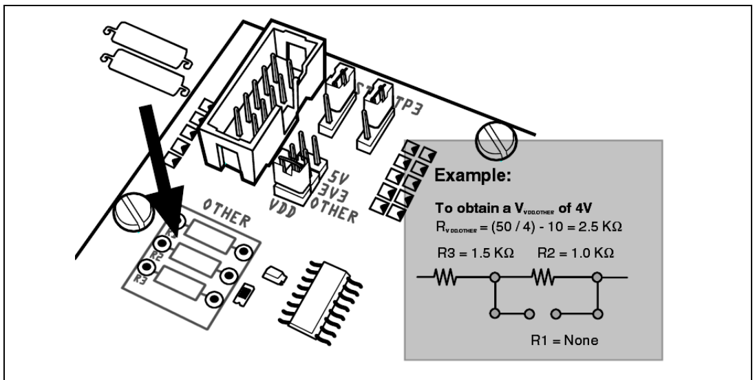
Figure 3: Installing serial resistors
