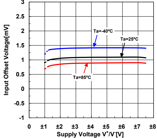
Input Offset Voltage vs. Supply Voltage (Temperature) V_{CM}=0\text{V}
